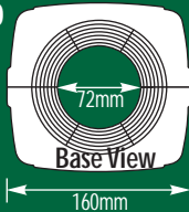
DOWNLIGHT GUARD MODEL No. I 721 72mm Cut-out Trim up to 114mm (2 piece assembly)
